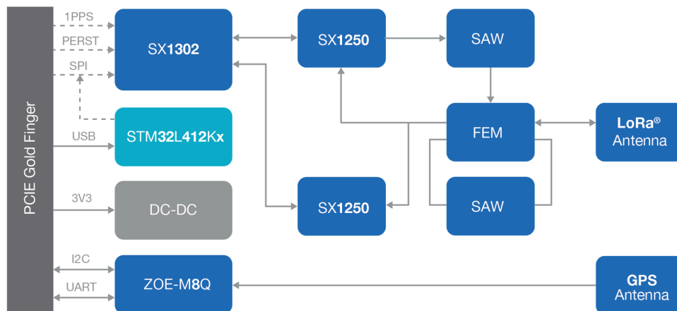
Figure 2: RAK2287 Block Diagram
