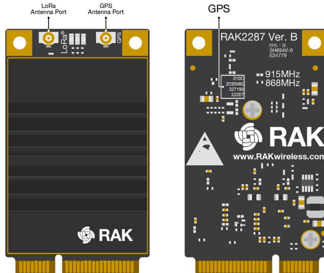
Figure 1: RAK2287 Board Overview
