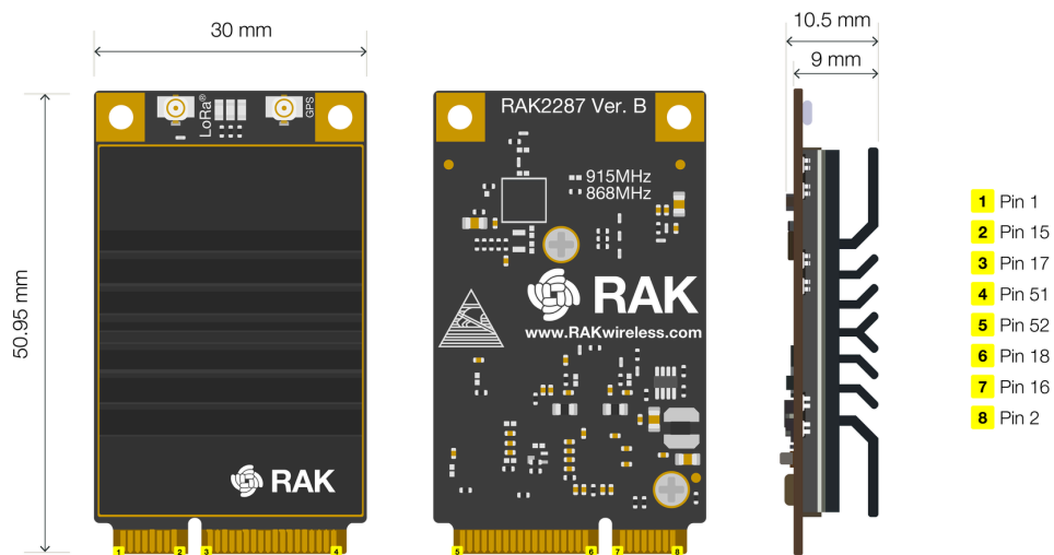
Figure 4: RAK2287 Board Dimensions
