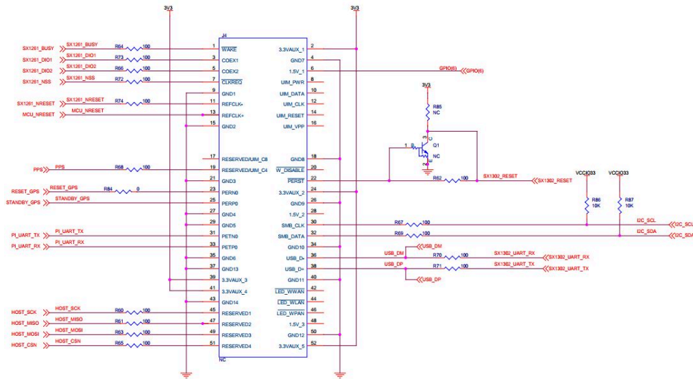
Figure 5: Schematic Diagram of RAK2287
